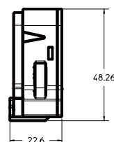
RIGHT1
